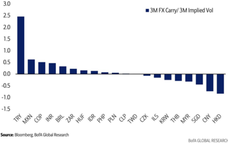
Exhibit 2: The TRY offers the best carry-to-vol ratio among all EM currencies The global backdrop is also supportive for EM carry trades now, in our view
